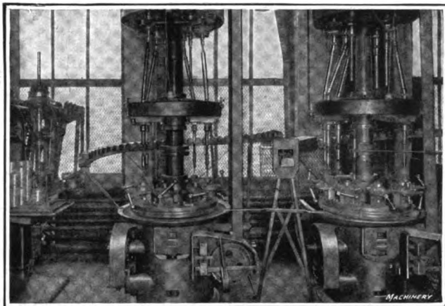
Fig. 14—In performing a sequence of operations on pistons, the Cadillac Motor Car Co. uses a trough in which the pistons are rolled from machine to machine. When an operation has been completed, the piston is removed from the machine and placed in the trough
